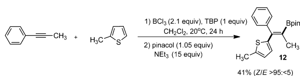
Scheme 6. Intermolecular 1,2-carbaboration.
